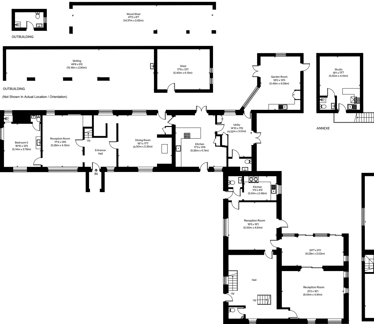
DAIRY GROUND FLOOR
